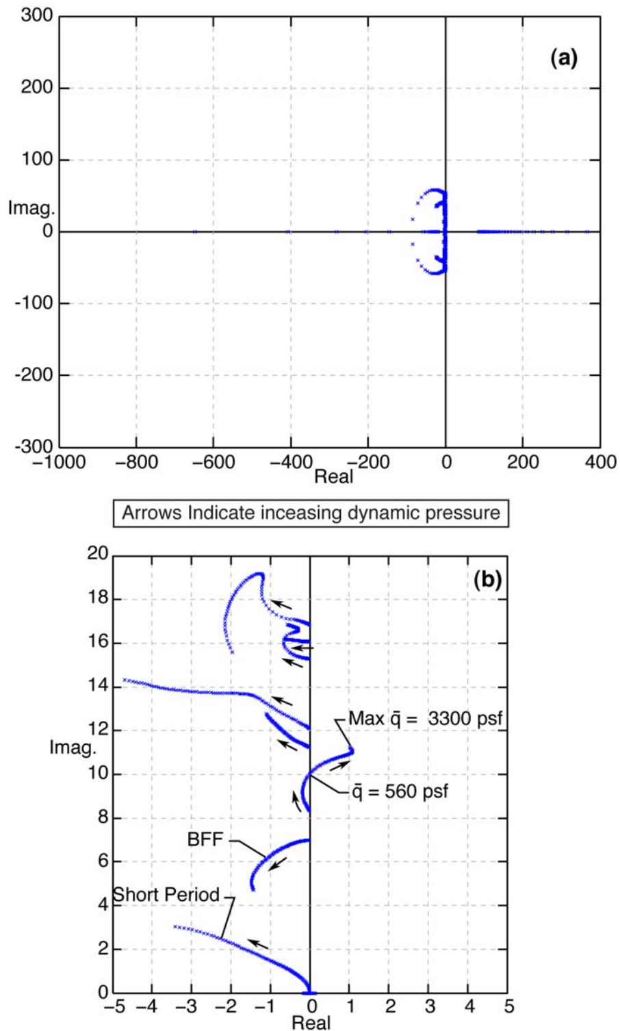
Figure 8. Root locus plot of flutter analysis with s-plane method using third-order matrix polynomial approximation of the unsteady aerodynamics at M = 0.8 .
