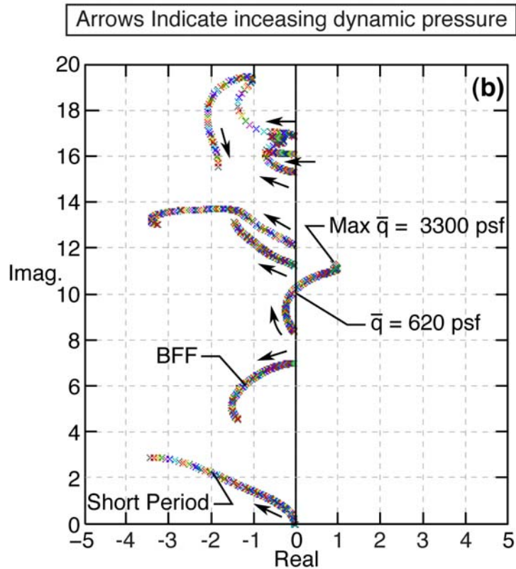
Figure 4. Root locus plot of flutter analysis with s-plane using ISAC-Roger's approximation aerodynamics at Mach = 0.8.
