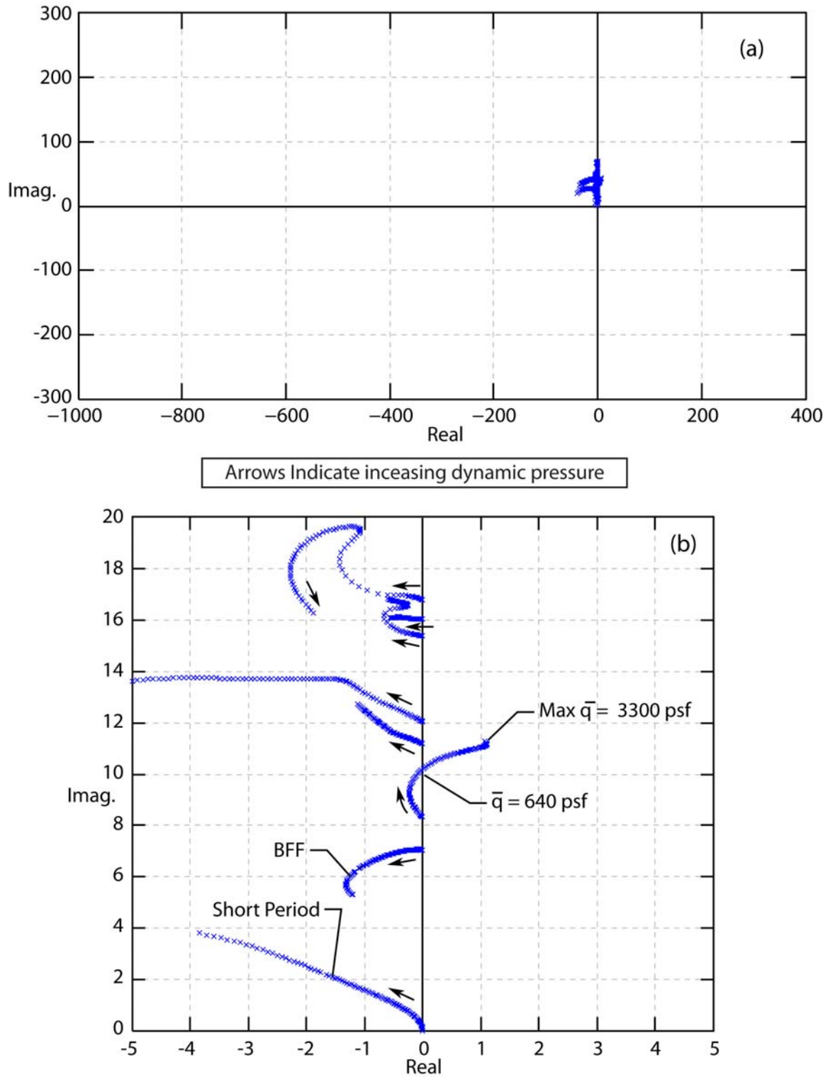
Figure 2. Root locus plot using NASTRAN pkn1 Flutter Analysis at M = 0.8 .
