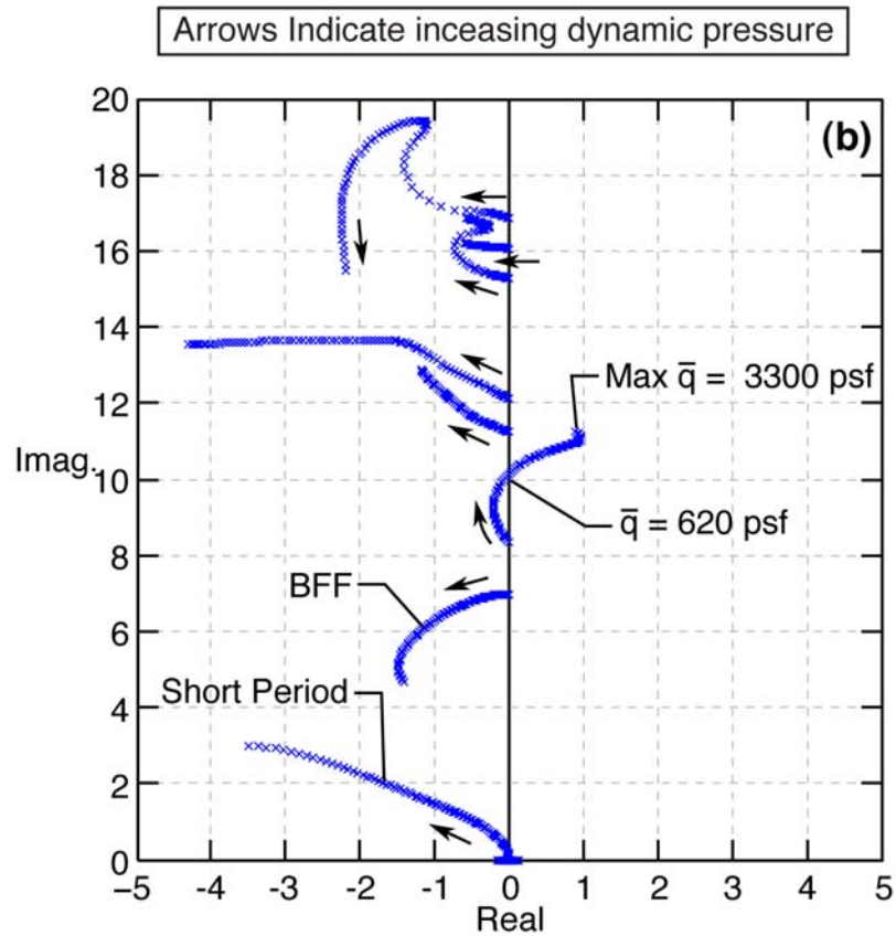
Figure 6. Root locus plot of flutter analysis with s-plane method using 20 th -order matrix polynomial approximation of the unsteady aerodynamics at M = 0.8 .
